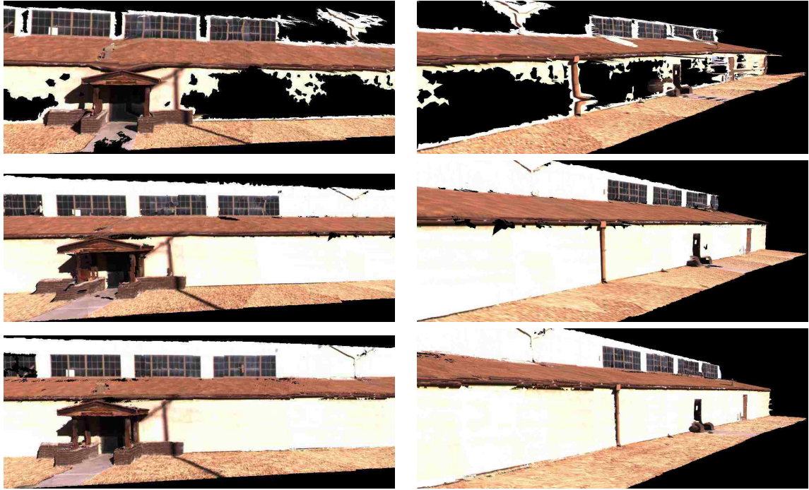
Figure 4.7: Screen shot of the 3D models. top: Window-based stereo. middle: Plane-fitting stereo. bottom: BP-based plane-fitting stereo.
