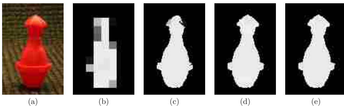
Figure 5.5: Intermediate results from iterative color-weighted refinement module. (a) Camera image. (b) The initial depth map ( D_0 ). (c) Depth map after one iteration ( D_1 ). (d) Depth map after three iterations ( D_3 ). (e) Depth map after ten iterations ( D_{10} ).
